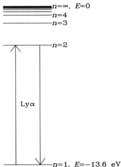
Figure 2.5 Energy levels of the hydrogen atom. Arrows indicate excitation from the ground state ( n = 1 ) to the first excited energy level ( n = 2 ), and deexcitation back to the ground state. Such excitation and deexcitation could be caused by, e.g., absorption by the atom of a Lyman- \alpha photon, and subsequent spontaneous emission of a Lyman- \alpha photon.
