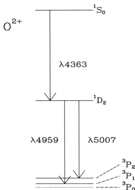
Figure 5.6 Part of the energy-level structure of the \text{O}^{2+} ion, an important cooling agent of interstellar gas. Radiative decay from the ^1\text{D}_2 state to two of the sublevels of the triply split ground state produces the emission-line doublet [O III] \lambda\lambda 4959, 5007 . (Decay to the third sublevel, ^3\text{P}_0 , is strongly forbidden.) For clarity, the spacing between the split levels has been greatly exaggerated. The [O III] \lambda 4363 emission line, resulting from radiative decay from ^1\text{S}_0 to ^1\text{D}_2 , can become strong in gas with a temperature high enough to excite a significant fraction of the ions to the ^1\text{S}_0 state.
