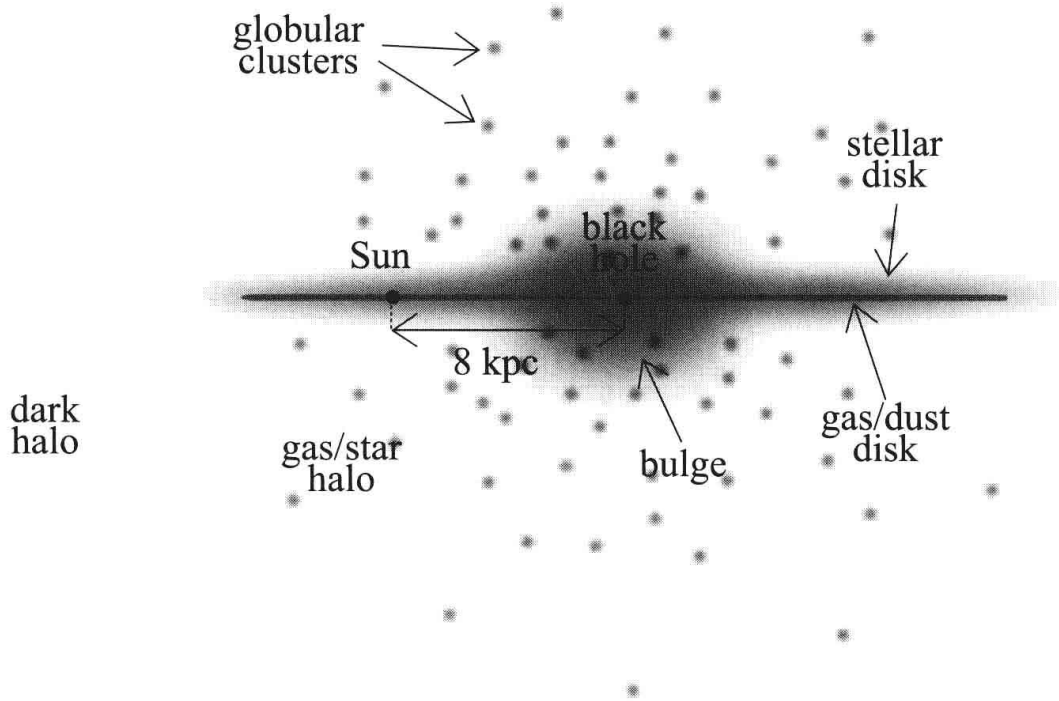
Figure 6.2 Schematic edge-on view of the main components of a spiral galaxy. The location of the Sun in the Milky Way is indicated.
