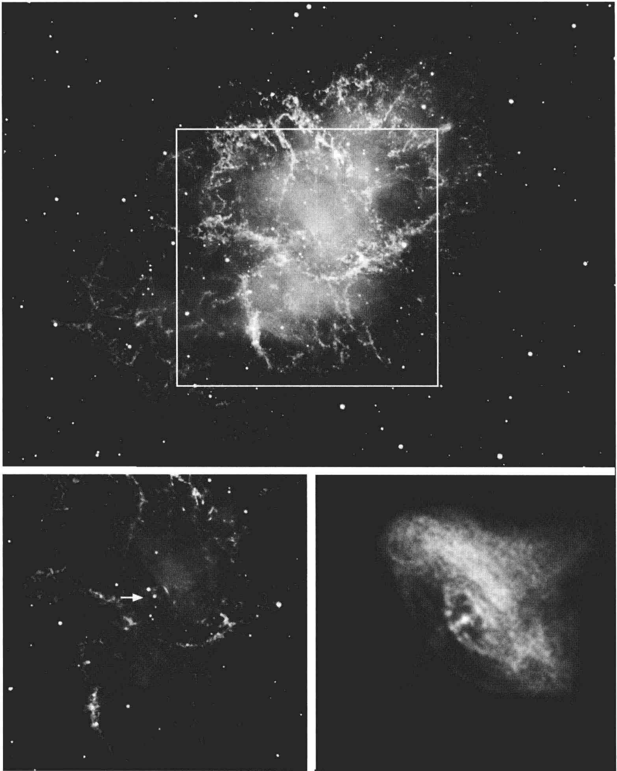
Figure 4.10 The Crab nebula, the remnant of a core-collapse supernova that exploded in the year 1054, at a distance of 2 kpc. Top: Image in optical light. Image scale is 4 pc on a side. Bottom: Zoom in on the area marked in the top photo, in optical light (left), with the pulsar at the center of the remnant indicated by the arrow; and in X-rays (right), showing the pulsar, bidirectional jets, and a toroidal structure formed by synchrotron emission from energetic particles. Note that a similar emission morphology is faintly discernible also in the optical image on the left. Photo credits: European Southern Observatory; and NASA/CXC/ASU and J. Hester et al.
