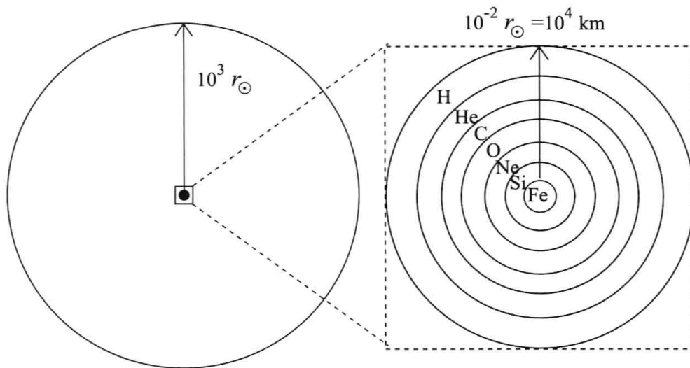
Figure 4.6 Simplified schematic view of the layered structure of a massive star and the distribution of the main elements that compose it, at the onset of core collapse and the ensuing supernova explosion.
