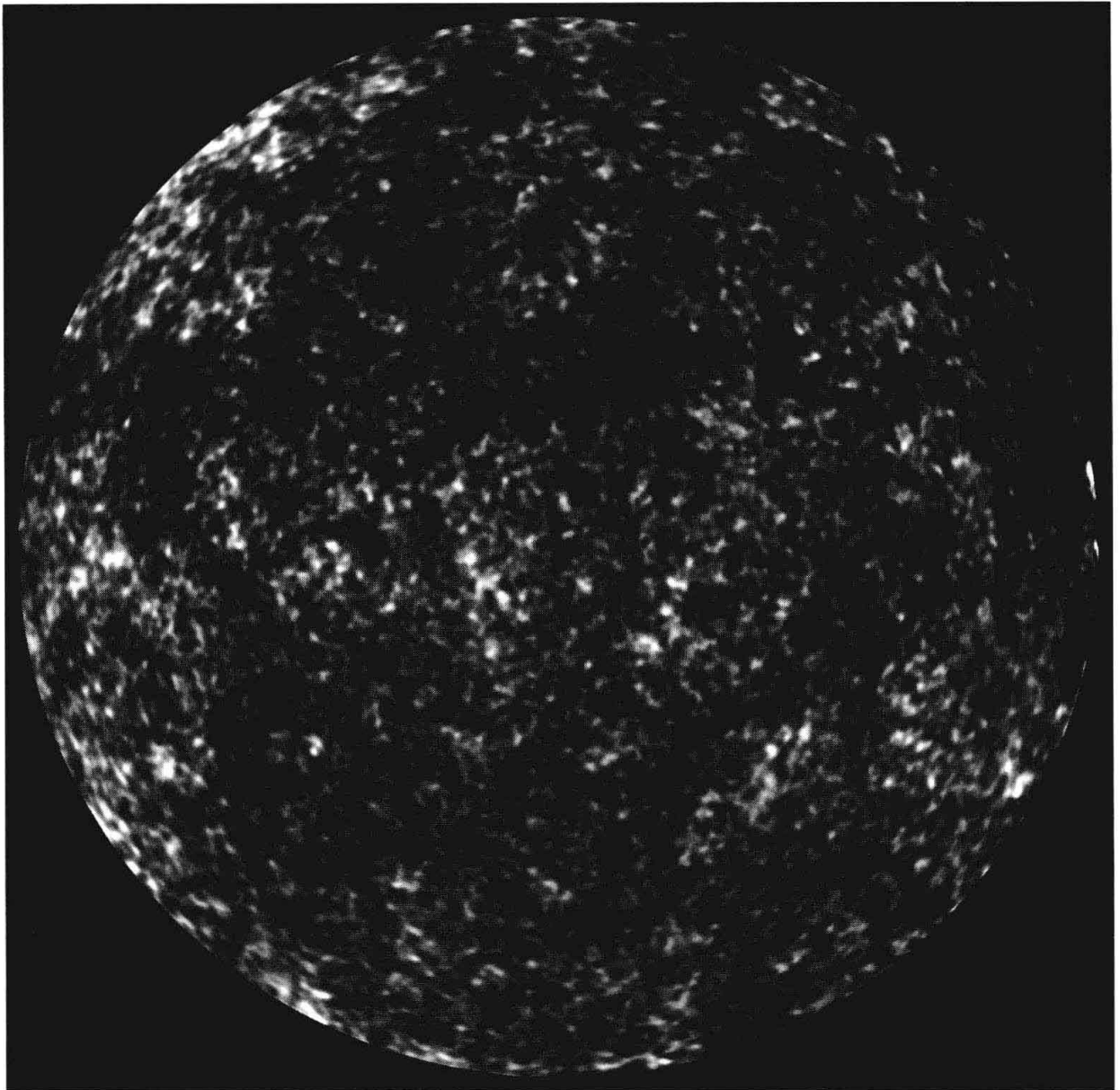
Figure 9.4 A half-sky ( 2\pi steradians) map of the temperature of the CMB sky. The typical relative fluctuations in the temperature, as coded by the gray scale (white is hot, black is cold), are of order 10^{-5} . Note the characteristic sizes of the hot and cold spots, \approx 0.4^\circ . As described in the text, this size provides a “standard ruler” with which the geometry of space can be measured. Foreground microwave emission from the Milky Way has been subtracted from the image, as well as the CMB “dipole” anisotropy due to the motion of the Local Group relative to the comoving cosmological frame. Photo credit: NASA and the WMAP Science Team.
