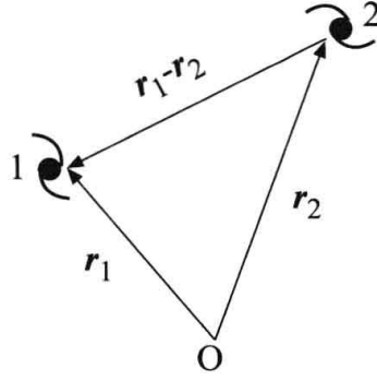
Figure 7.7 An observer at O sees galaxies at vector positions \mathbf{r}_1 and \mathbf{r}_2 receding according to Hubble's law. Observers in each of those galaxies will see the other two galaxies receding from them according to the same Hubble law.
