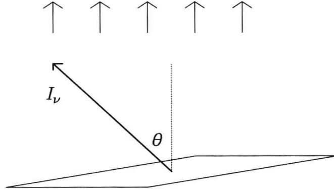
Figure 2.2 Illustration of the net flux emerging through surface of a blackbody, due to a beam with intensity I_\nu emerging at an angle \theta to the perpendicular.
