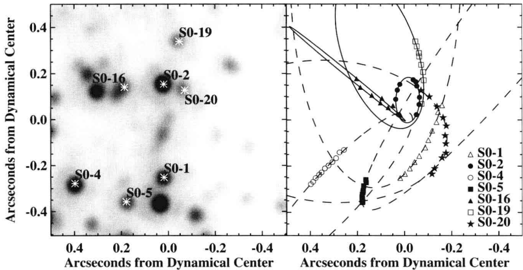
Figure 6.5 Left: Near-infrared (2.2-μm-wavelength) diffraction-limited image of the central arcsecond (0.04 pc) around the Galactic center, obtained in June 2005. Right: Positions of the seven stars marked in the left panel, as traced with such images between 1995 and 2005, and the best-fitting elliptical orbits. The orbits indicate an enclosed mass of \approx 4 \times 10^6 M_{\odot} within a radius of < 45 AU (the closest approach achieved by star S0-16), presumably a supermassive black hole at the position of Sagittarius A*. Figure credit: A. Ghez and J. R. Lu, see Astrophys. J. (2005), 620, 744.
