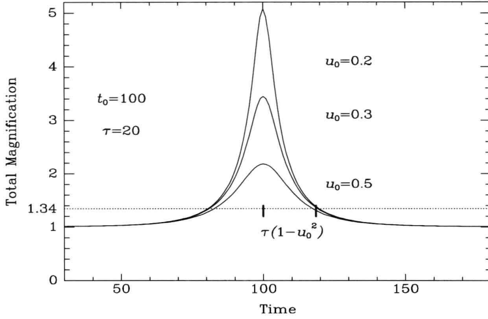
Figure 6.12 Theoretical microlensing curves, obtained by combining Eqs. 6.32 and 6.37, and showing the total magnification of a microlensing event as a function of time. Curves are shown for three different Einstein-angle-normalized impact angles u_0 . The time of maximal approach is t_0 = 100 and the Einstein-crossing timescale is \tau = 20 (both in arbitrary time units). Note how the peak magnification rises with decreasing u_0 , and equals approximately u_0^{-1} , as expected from Eq. 6.35.
