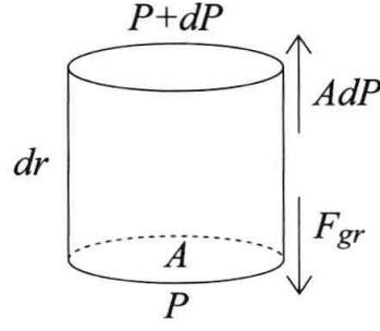
Figure 3.1 Hydrostatic equilibrium. The gravitational force F_{gr} on a mass element of cross-sectional area A is balanced by the force AdP due to the pressure difference between the top and the bottom of the mass element.
