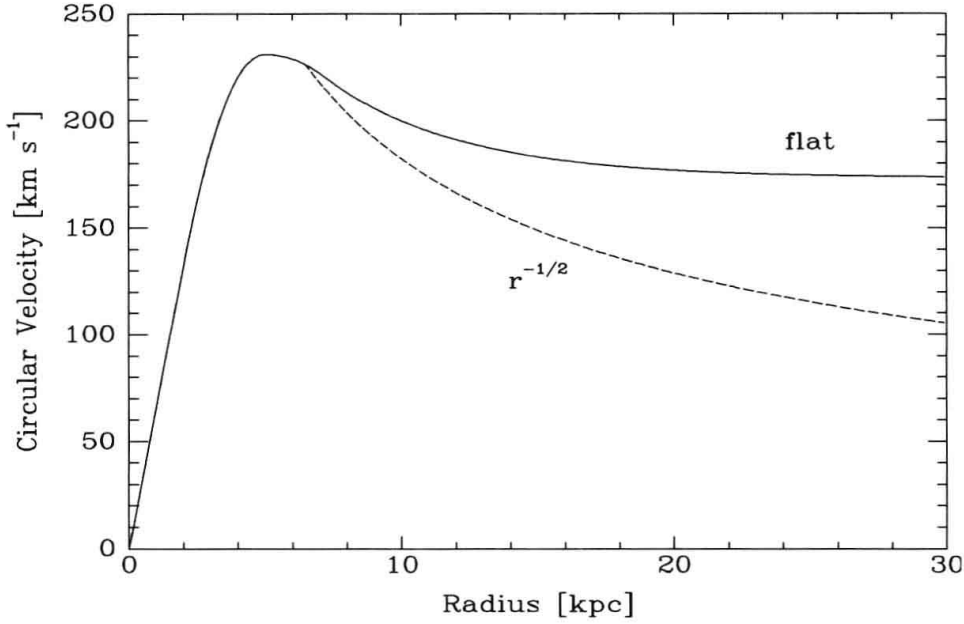
Figure 6.6 Schematic example of a spiral galaxy’s rotation curve—its circular velocity as a function of radius. Outside the inner few kiloparsecs, rotation curves invariably become “flat,” i.e., approach a constant velocity, suggesting the presence of a halo of dark matter. The dashed curve shows the \sim r^{-1/2} Keplerian falloff that would be expected, in the absence of dark matter, beyond a radius that includes most of the visible luminous matter.
