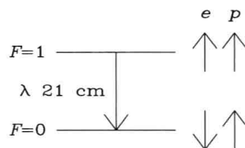
Figure 5.8 The hyperfine-split ground state of hydrogen. The lower level has angular momentum F = 0 , corresponding to antiparallel electron and proton spins, and the upper level has F = 1 , with the two spins parallel. In a radiative decay between the levels, the spin of the electron flips, and a \lambda = 21 cm ( \nu = 1421 MHz, h\nu = 5.9 \times 10^{-6} eV) photon is emitted.
