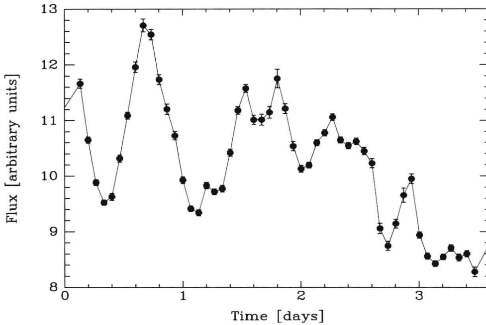
Figure 6.20 Flux variations in the 2- to 10-keV X-ray band of the active galactic nucleus NGC 3516, over several days. Note the large variation amplitudes on timescales of hours, and the nonperiodic, random nature of the variability. Data credit: A. Markowitz and R. Edelson 2005, Astrophys. J. , 617, 939.
