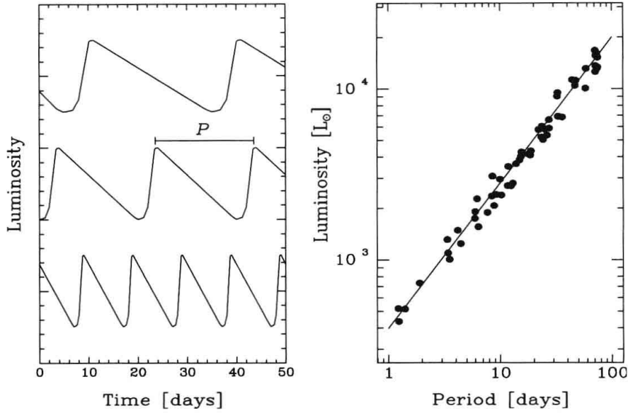
Figure 7.1 Illustration of Cepheid properties. Left: Schematic time series for Cepheids of different luminosities. Right: Schematic Cepheid period-luminosity relation. Once the relation is calibrated for nearby Cepheids, it can be used to determine the luminosity of Cepheids with measured periods in another galaxy. Comparison of the derived luminosity to the observed Cepheid flux then yields the distance to the galaxy.
