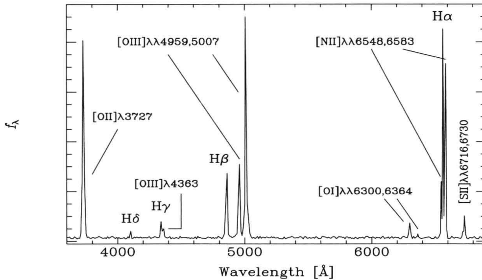
Figure 5.7 Typical optical spectrum of an H II region, with the main emission lines marked—the Balmer series from hydrogen recombination, and the collisionally excited “metal” lines.
