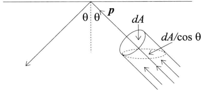
Figure 3.6 Calculation of radiation pressure. A beam of photons with blackbody intensity B strikes the wall of a container at an angle \theta to its perpendicular. The projected area of the beam, dA , is increased by 1/\cos \theta , and therefore the power reaching the wall per unit area is decreased to B \cos \theta . Since a photon's momentum, p , is its energy divided by c , the momentum flux in the beam is B/c . Every reflection of a photon transfers twice its perpendicular component of momentum, and therefore the momentum transfer per unit time and per unit area, i.e., the pressure, is 2B \cos^2 \theta/c . The total pressure is obtained by integrating over all angles of the beams that approach the wall.
