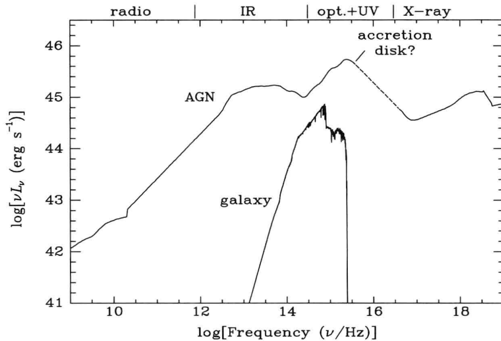
Figure 6.19 Typical spectral energy distribution of an active galactic nucleus, from radio to X-ray frequencies. The vertical axis shows \nu L_\nu(\nu) , which has units of luminosity, and which is convenient for visualizing the relative luminosities in different frequency bands. The much-narrower spectral energy distribution of stars in a typical galaxy is shown for comparison. The indicated “bump” in the optical-to-UV range in the AGN spectral distribution may be due to thermal radiation from an accretion disk around the central black hole. The dashed section of the curve is an interpolation in the extreme-UV band, where observations are difficult, because of strong absorption of light from extragalactic sources by neutral hydrogen in the interstellar medium of the Milky Way. Data credit: M. Elvis et al. 1994, Astrophys. J. Suppl. , 95, 1.
