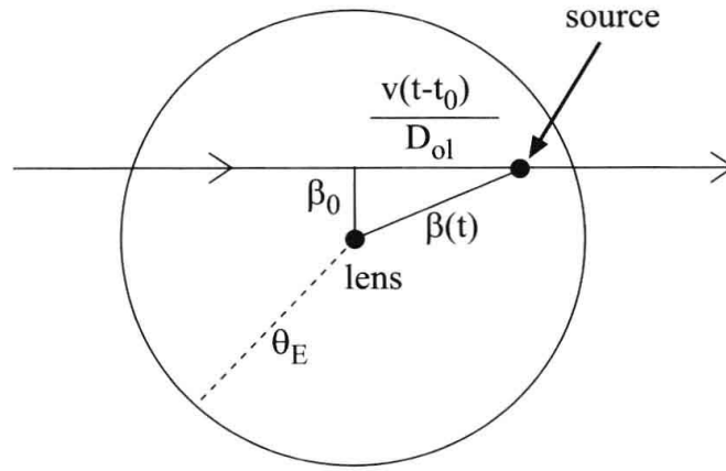
Figure 6.11 Relative motion on the sky of a lens (center, with its Einstein angle \theta_E indicated) and a source that is projected behind it. Projected to the plane of the lens, the source moves at a constant transverse velocity v in a straight line, with an angle of closest approach \beta_0 at time t_0 . From the Pythagorean theorem, the time dependence of the lens–source separation, \beta(t) , is given by Eq. 6.36.
