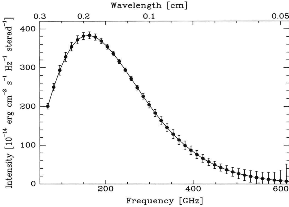
Figure 9.3 Observed spectrum of the cosmic microwave background, compared with a T = 2.725 -K blackbody curve. The error bars shown are 500\sigma , so as to be discernible in the plot. Data credit: D. J. Fixsen et al. 1996, Astrophys. J. , 473, 576.
