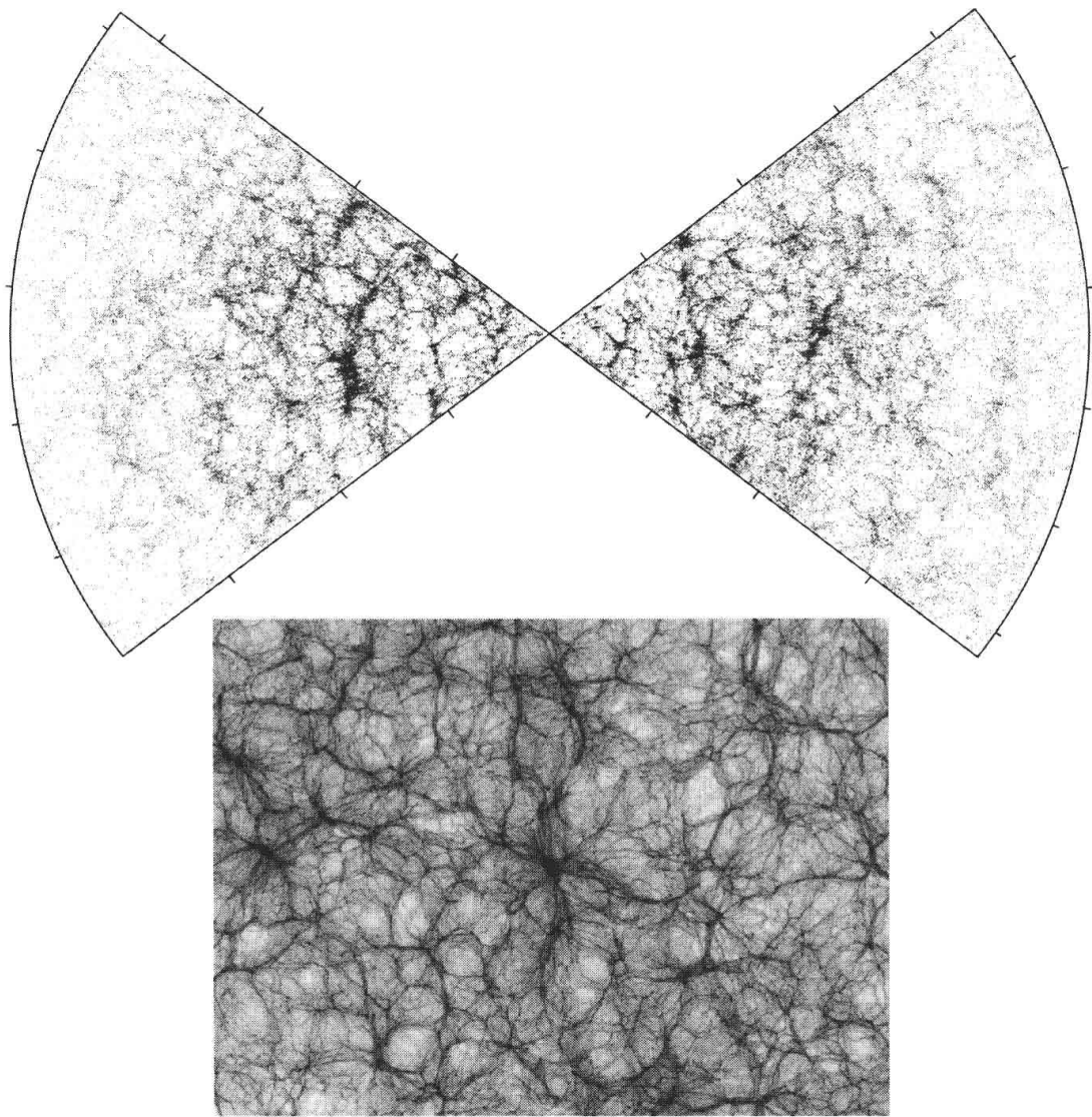
Figure 6.22 Top: The space distribution of galaxies, as observed in two thin slices that are centered on our location in the Universe (every dot represents a galaxy). The figure was produced by measuring the two-dimensional positions of the galaxies in two narrow, diametrically opposed, strips on the sky, and the distance to each galaxy. Note the large aggregations of galaxies which surround relatively empty “void” regions. Every tick mark in the radial direction corresponds to \sim 150 Mpc. The “thinning out” of points beyond \sim 400 Mpc is an observational effect—at these distances, only the rare, more luminous, galaxies are bright enough to have their distances measured accurately. Bottom: A slice through the volume of a numerical N-body simulation in which 10^{10} particles move under the influence of their mutual gravitational attractions. Each particle in the calculation represents a mass of \sim 10^9 M_{\odot} , and the image width is about 500 Mpc. Note the web-like distribution of particles, which is reminiscent of the observed galaxy distribution in the top figure. Figure credits: The 2dF Galaxy Redshift Survey team, see M. Colless et al. 2001 & 2003, http://arXive.edu/abs/astro-ph/0306581 ; and V. Springel and the Millenium Simulation team, see Nature , 435 (2005), 629.
