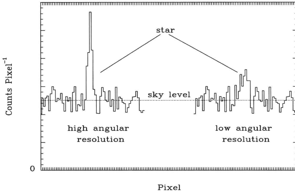
Figure 1.4 Cuts through the positions of a star in two different astronomical images, illustrating the effect of angular resolution on the detectability of faint sources on a high background. The vertical axis shows the counts registered in every pixel along the cut, as a result of the light intensity falling on that pixel. On the left, the narrow profile of the stellar image stands out clearly above the Poisson fluctuations in the sky background, the mean level of which is indicated by the dashed line. On the right, the counts from the same star are spread out in a profile that is twice as wide, and hence the contrast above the background noise is lower.
