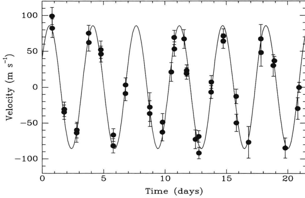
Figure 2.11 Observed radial velocity curve (i.e., line-of-sight velocity vs. time) for the nearby ( \approx 50 pc) star HD209458, revealing the presence of a planetary companion that causes the star to orbit around the common center of mass. Using Eq. 2.45, and assuming the parent star has a mass M_1 = 1.1M_\odot (based on its observed spectral type), the amplitude ( 86 \text{ m s}^{-1} ) and period (3.5 days) of the observed velocity oscillations indicate a planet mass M_2 = 0.7M_J / \sin i , where M_J is one Jupiter mass. The orbital radius is 0.05 AU. In this particular system, a periodic 1.5% amplitude eclipse of the star’s flux has also been detected, due to the transit of the planet across the face of the star, indicating \sin i \approx 1 . Data credit: T. Mazeh et al. 1999, Astrophys. J. , 532, L55.
