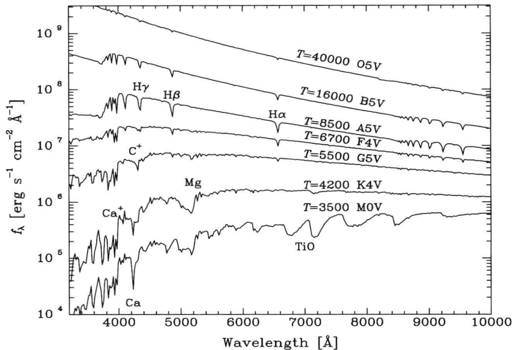
Figure 2.6 Zoom-in on the optical wavelength region of the stellar spectra shown in Fig. 2.1. The curves are labeled with their spectral types, in addition to the corresponding blackbody temperatures, which constitute the effective temperatures of the stars. Note the various labeled absorption features that appear and disappear as one goes from one spectral type to another. Data credit: R. Kurucz.
