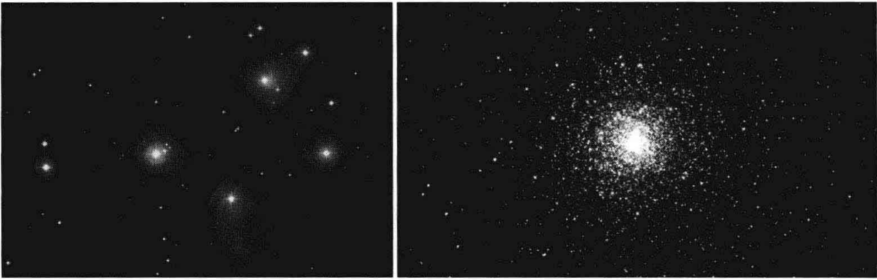
Figure 5.2 Left: The Pleiades, an open star cluster that is visible to the naked eye, at a distance of 120 pc. Note the nebulosities surrounding some of these young stars. Image scale is about 2 pc on the vertical side. Right: The globular cluster M80, at a distance of 8.7 kpc. Image scale is 4 pc on the vertical side. Photo credits: NASA, ESA, AURA/Caltech; NASA and the Hubble Heritage Team.
