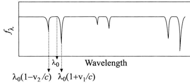
Figure 2.8 Schematic example of the spectrum of a double-lined spectroscopic binary. Each of the absorption lines in the spectrum appears twice, Doppler-shifted to longer and shorter wavelengths, respectively, as a result of the orbital motion of the binary members about their center of mass. During the orbital period, each absorption line oscillates back and forth about the restframe wavelength \lambda_0 .
