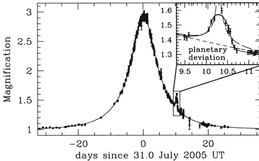
Figure 6.14 Example of a microlensing event observed in the direction of the Galactic bulge, involving a foreground star that temporarily magnifies the light from a background star projected behind it. Note the excellent fit (solid curve) to the data provided by Eqs. 6.32 and 6.37 during most of the event. However, the small, day-long, perturbation in the curve of magnification vs. time on its falling side (enlarged in the inset) reveals the presence of a planet around the lens star. A detailed model (solid curve in the inset) indicates an approximately 5-Earth-mass planet at an orbital radius of several AU from the main lens star. The single-lens model (short-dashed curve) and a model assuming a binary source star (long-dashed curve) are both ruled out by the data. Figure credit: PLANET, OGLE, and MOA collaborations, see J.-P. Beaulieu et al. 2006, Nature , 439, 437.
