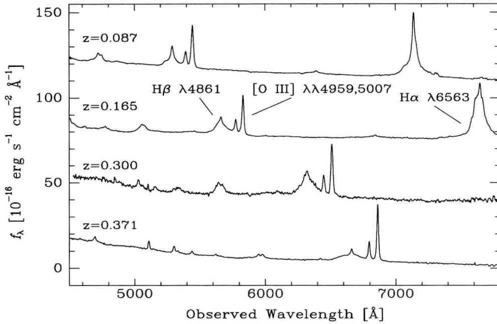
Figure 9.1 Optical spectra of four quasars, with cosmological redshifts increasing from top to bottom, as marked. Note the progression to the red of the main emission lines, which are indicated. The width of the Balmer lines is the result of Doppler blueshifts and redshifts about the line centers, due to internal motions of the emitting gas, under the influence of the central black holes powering the quasars. The [O III] lines are narrower because they are emitted by gas with smaller internal velocities. Data credit: S. Kaspi et al. 2000, Astrophys. J. , 533, 631.
