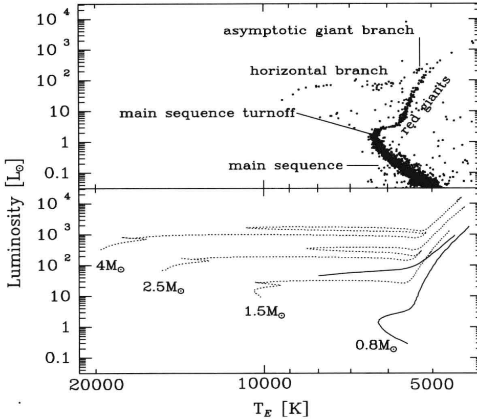
Figure 4.1 Illustration of post-main-sequence evolution on the H-R diagram. Top: Observed H-R diagram for stars in the globular cluster M3 (more on star clusters in section 5.1.5). The main-sequence turnoff marks the point at which stars are now leaving the main sequence and evolving on to the red-giant branch. All the stars in the cluster formed together about 13 Gyr ago, and the cluster has not experienced subsequent star formation. As a result, all stars above a certain mass, corresponding to the turnoff point, have left the main sequence, while those below that mass are still on the main sequence. The density of points in each region of the diagram reflects the amount of time spent by stars in each post-main-sequence evolution stage. Bottom: Theoretical stellar evolution tracks for stars of various initial main-sequence masses (with an assumed initial metal abundance of Z = 0.0004 ). Each track begins at the lower left end on the zero-age main sequence . After leaving the main sequence, stars evolve along, and up to the tip of, the red-giant branch. They then move quickly on the diagram to the left edge of the horizontal branch , where helium core burning and hydrogen shell burning take place, and evolve to the right along the horizontal branch. Once all the helium in the core has been converted to carbon and oxygen, the star rises up the “asymptotic giant branch” where double shell burning—a helium-burning shell within a hydrogen burning shell—takes place. Note the good correspondence between the theoretical track for the 0.8M_{\odot} initial-mass star (solid line) and the observed H-R diagram on top. For clarity, the theoretical horizontal and asymptotic giant branches are not shown for the other initial masses. Data credits: S.-C. Rey et al. 2001, Astrophys. J. , 122, 3219; and L. Girardi, et al. 2000, Astron. Astrophys. Suppl. , 141, 371.
