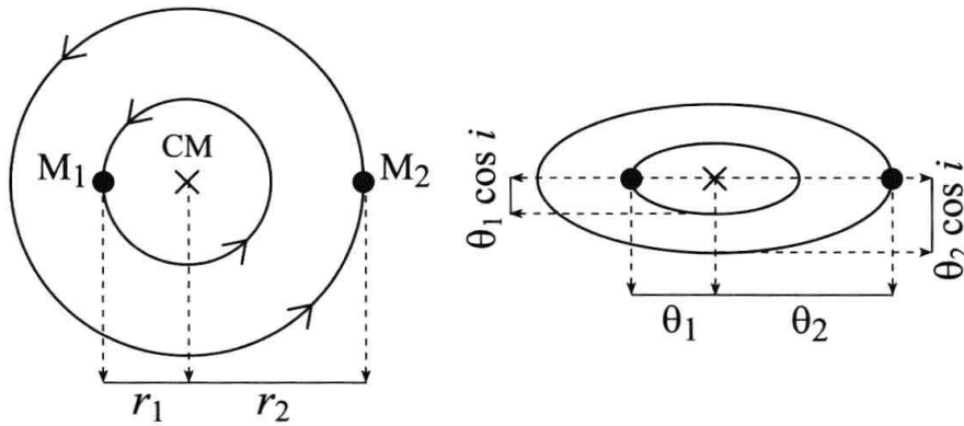
Figure 2.9 Left: A binary system, viewed pole-on, with its members in circular orbits with physical radii r_1 and r_2 around their common center of mass. Right: The appearance of the system when viewed as a visual binary, with the orbital plane inclined by an angle i to the line of sight, and orbital radii subtending angles on the sky \theta_1 and \theta_2 . The circular orbits now appear as ellipses, with minor axes foreshortened by \cos i .
