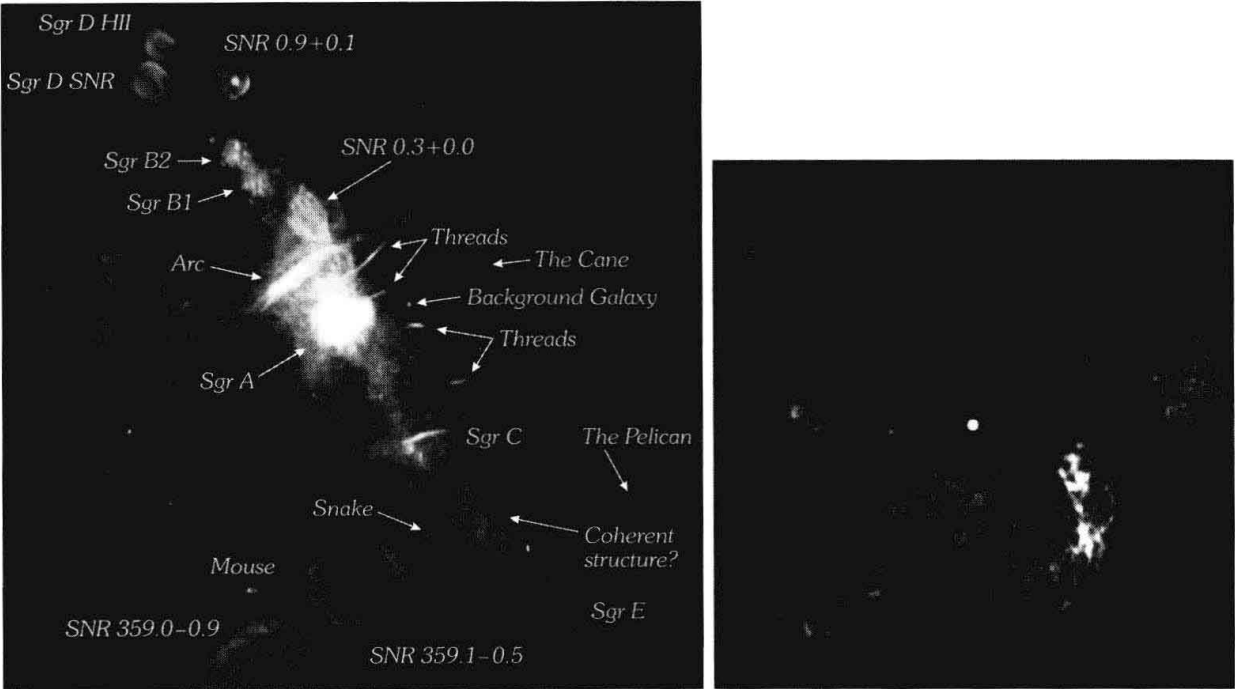
Figure 6.4 Left: A radio-wavelength (90 cm) image of \sim 1 kpc around the Galactic center. The Galactic plane goes from top-left to bottom-right (compare to Fig 6.3). The central source radio source, Sagittarius A, is marked. The unresolved radio source at the kinematic center of the Galaxy, Sagittarius A*, is within it. A number of other structures are also identified, mainly supernova remnants emitting synchrotron radiation and H II regions that emit free-free radiation. Right: Radio image at a wavelength of 1.3 cm of the central parsec around Sagittarius A*, which is at the center of the image, surrounded by diffuse emission from ionized gas. Photo credits: NRAO/AUI and N. E. Kassim, Naval Research Laboratory; NRAO/AUI, Jun-Hui Zhao, and W. M. Goss.
