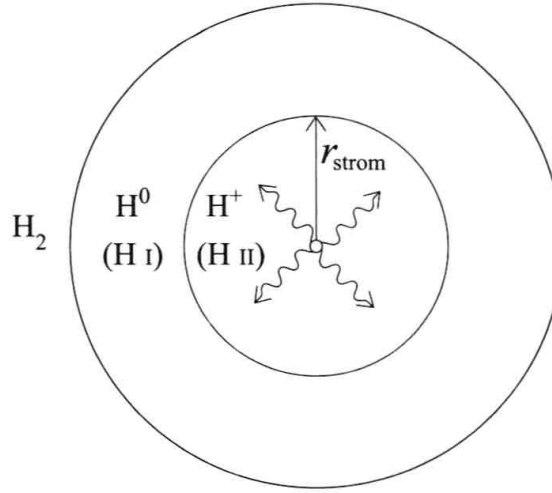
Figure 5.3 Schematic illustration of the Strömgren sphere of ionized hydrogen that is produced around a hot star via photoionization. Inside the radius r_{\text{strom}} , the hydrogen is almost completely ionized, i.e., there is an “H II” region. Beyond r_{\text{strom}} , the hydrogen is neutral (“H I”), since all photons capable of ionizing it have been absorbed. Further yet from the star, all photons energetic enough to photodissociate hydrogen molecules, \text{H}_2 , have also been absorbed, and the gas is molecular.
