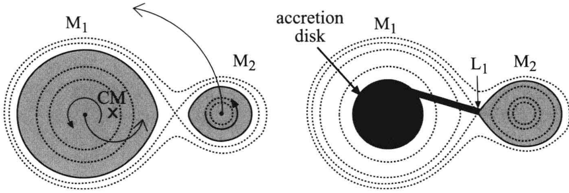
Figure 4.12 Equipotential surfaces (dotted curves) in the corotating reference frame of a binary system with mass ratio M_1/M_2 = 5 . Left: In this example, both stars are inside their respective Roche lobes, but are tidally distorted. Loss of energy to tidal friction will cease only when the orbits about the center of mass become circularized, and aligned and synchronized with the rotations, so that there is no motion in the corotating frame. Right: Here, the secondary star, on the right, fills its Roche lobe. Matter flows through the L_1 point and falls onto the primary star, which is now a compact object. Viewed from an inertial frame, the falling material possesses angular momentum, and hence an accretion disk is formed around the compact primary star.
