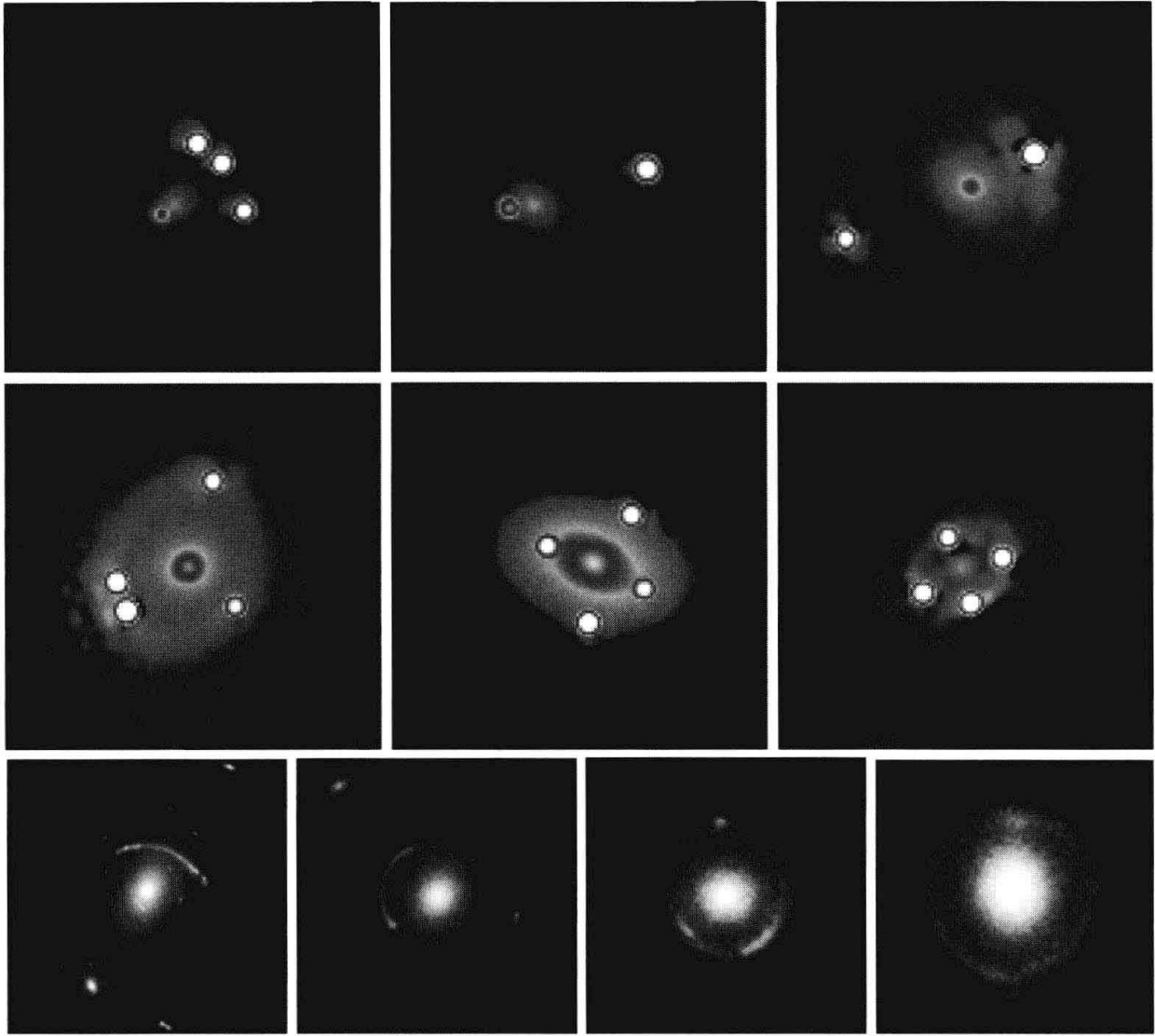
Figure 9.8 Top two rows: Examples of quasars that are gravitationally lensed into multiple images by intervening galaxies. In each case, the lens galaxy, at a redshift of z \approx 0.04\text{--}0.7 , is the extended central object, and the two or four sources straddling it are the multiply lensed images of a background quasar, at z \approx 1.7\text{--}3.6 . Panels are 5 arcseconds on a side. Some image processing has been applied, to permit seeing clearly both the bright, point-like, quasar images and the faint, extended lens galaxies. Bottom row: Examples of foreground galaxies that lens background galaxies into partial or full Einstein rings. In the cases shown, the foreground galaxies are at z \approx 0.2\text{--}0.4 and the background galaxies are at z \approx 0.5\text{--}1 . Photo credits: The CASTLES gravitational lens database, C. Kochanek et al.; NASA, ESA, J. Blakeslee and H. Ford,; and NASA, ESA, A. Bolton, S. Burles, L. Koopmans, T. Treu, and L. Moustakas.
