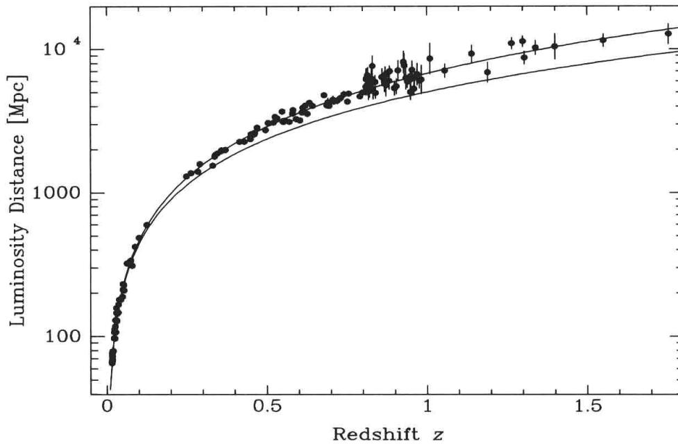
Figure 9.2 A Hubble diagram extending out to redshift z \approx 1.7 , based on type Ia supernovae. Note that redshift now replaces velocity (compare to Fig. 7.6) and the luminosity distances to these standard candles are now plotted on the vertical axis. The top and bottom curves give the expected relations for cosmologies with \Omega_m = 0.3 , \Omega_\Lambda = 0.7 , and \Omega_m = 1 , \Omega_\Lambda = 0 , respectively. The data favor the top curve, indicating a cosmology currently dominated by dark energy. The calculation of the curves is outlined in Problems 4–7. Data credits: A. Riess et al. 2004, Astrophys. J. , 607, 665, and P. Astier et al., 2006, Astron. Astrophys. , 447, 31.
