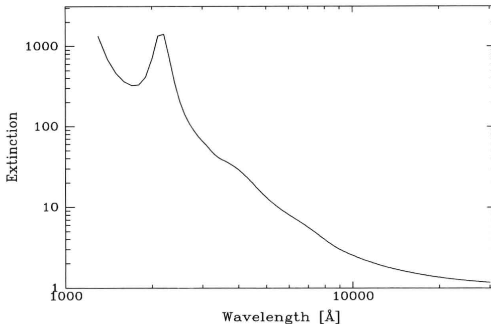
Figure 5.10 A typical curve of extinction—the attenuation factor produced by interstellar dust—as a function of wavelength, from the UV (1300 Å) to the near-IR (3 μm). The case shown is set to have a factor of 10 extinction at 5500 Å. Note the large extinctions in the UV, compared to the moderate values at IR wavelengths. Data credit: J. Cardelli et al. 1988, Astrophys. J. , 329, L33.
