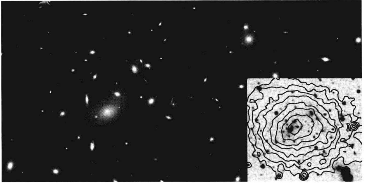
Figure 6.21 Optical image of the central region of the massive galaxy cluster Abell 2218. Note the preponderance of elliptical galaxies. The conspicuous arcs are gravitationally lensed images of distant background galaxies projected near the center of the cluster. The arcs are effectively partial Einstein rings, which allow a measurement on the total mass projected internal to them. Image width is about 0.6 Mpc. Inset: Contours showing the X-ray intensity from the cluster, superimposed on an optical image. The area within the inner three contours corresponds approximately to the area shown in the main high-resolution image. The X-ray emission is bremsstrahlung from hot intracluster gas bound by the gravitational potential of the cluster. The gas mass is an order of magnitude greater than the stellar mass of the cluster. The gas temperature provides an independent measure of the total cluster mass. Photo credits: NASA, A. Fruchter, and the ERO Team; and F. Govoni et al. 2004, Astrophys. J. , 605, 695, reproduced by permission of the AAS.
