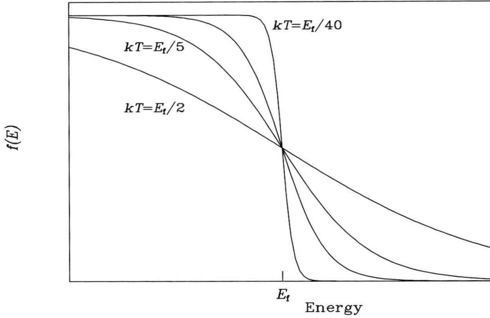
Figure 4.4 Approach to degeneracy of the Fermi-Dirac occupation number, f(E) , as kT \rightarrow 0 , shown for kT = E_f/2, E_f/5, E_f/10 , and E_f/40 . At kT \ll E_f , all particles occupy the lowest energy state possible without violating the Pauli exclusion principle. The distribution then approaches a step function, with all energy states below E_f occupied, and all those above E_f empty.
