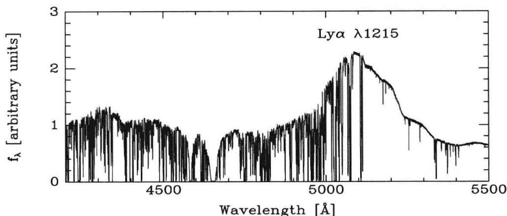
Figure 9.7 A high-resolution spectrum of a quasar at redshift z = 3.18 , with the Lyman \alpha emission line redshifted to 5080 Å. Note the Lyman- \alpha forest of absorption lines starting from the peak of the emission line, and continuing in the blue (left) direction. These lines are due to Lyman- \alpha absorption by neutral hydrogen atoms in gas clouds that are along the line of sight to the quasar, and hence at lower redshifts than the quasar. The few absorption lines to the red of the Lyman- \alpha emission line peak are due to heavier elements and are associated with the system that produces the strong damped Lyman- \alpha absorption observed at \approx 4650 Å. Data credit: W. Sargent and L. Lu, based on observations with the HIRES spectrograph at the W. M. Keck Observatory.
